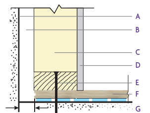
FIGURE 3 - Section – Murs non finis
