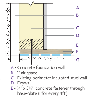
FIGURE 3 - Section - Unfinished Walls
