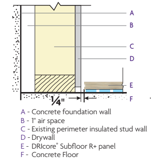
FIGURE 2 - Section - Finished Walls
