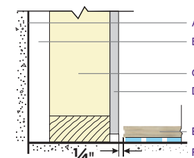
FIGURE 2 - Section – Murs finis
