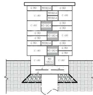
ELEVATION D
