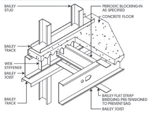
JOIST PARALLEL TO PERIMETER
