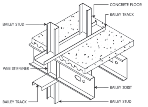
JOIST ABOVE LOADBEARING WALL
