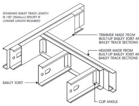
OPENING IN FLOOR
