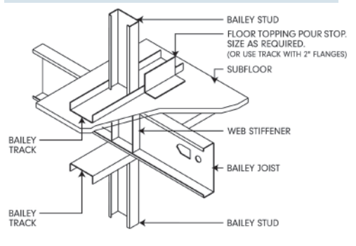
JOIST ABOVE LOADBEARING WALL
