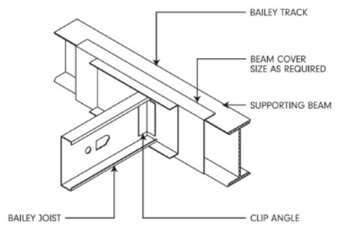
FLUSH CONNECTION TO SUPPORTING BEAM
