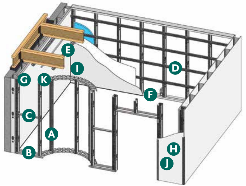
A NON LOAD BEARING STEEL STUD
